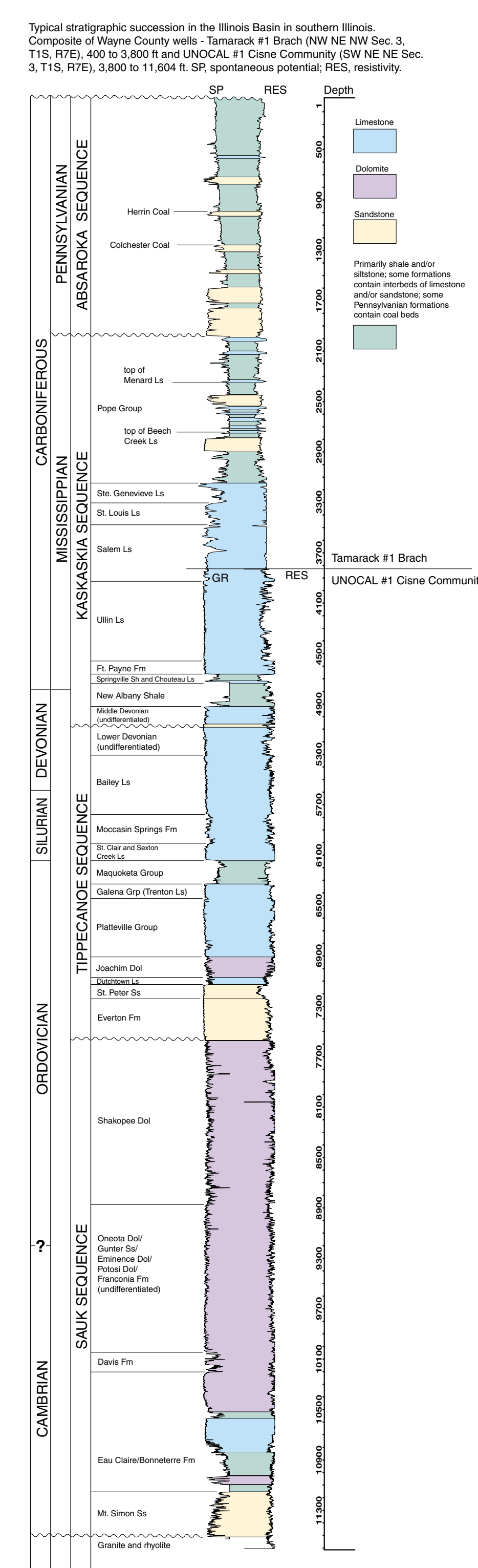
Wireline Logs
