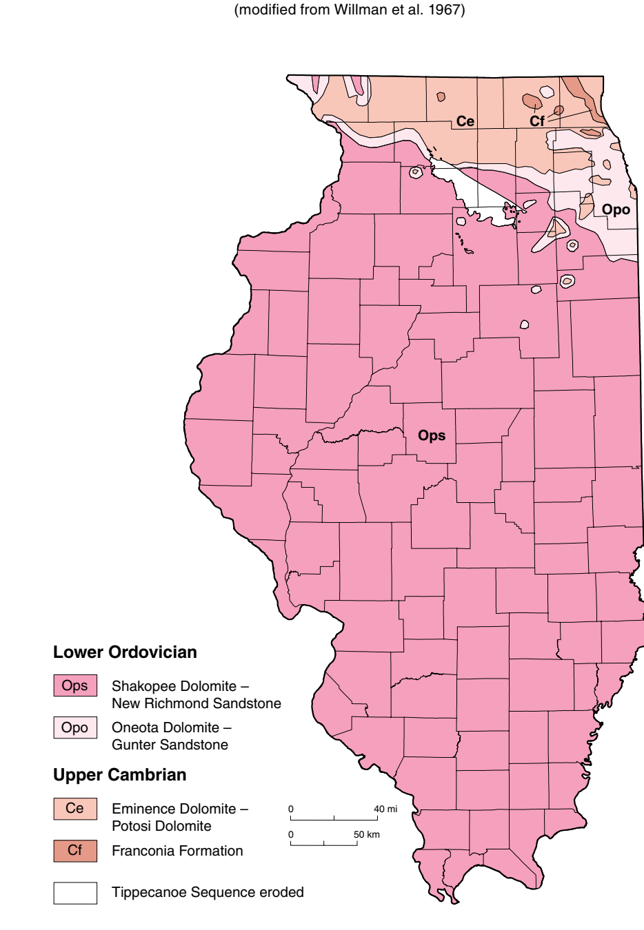
Sub-Tippecanoe Geologic Map
