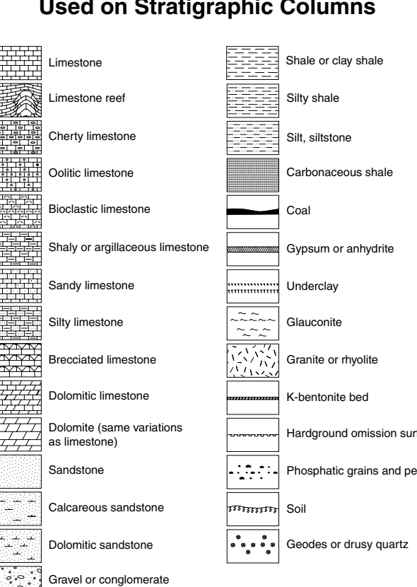
Explanation of Lithologic Symbols
