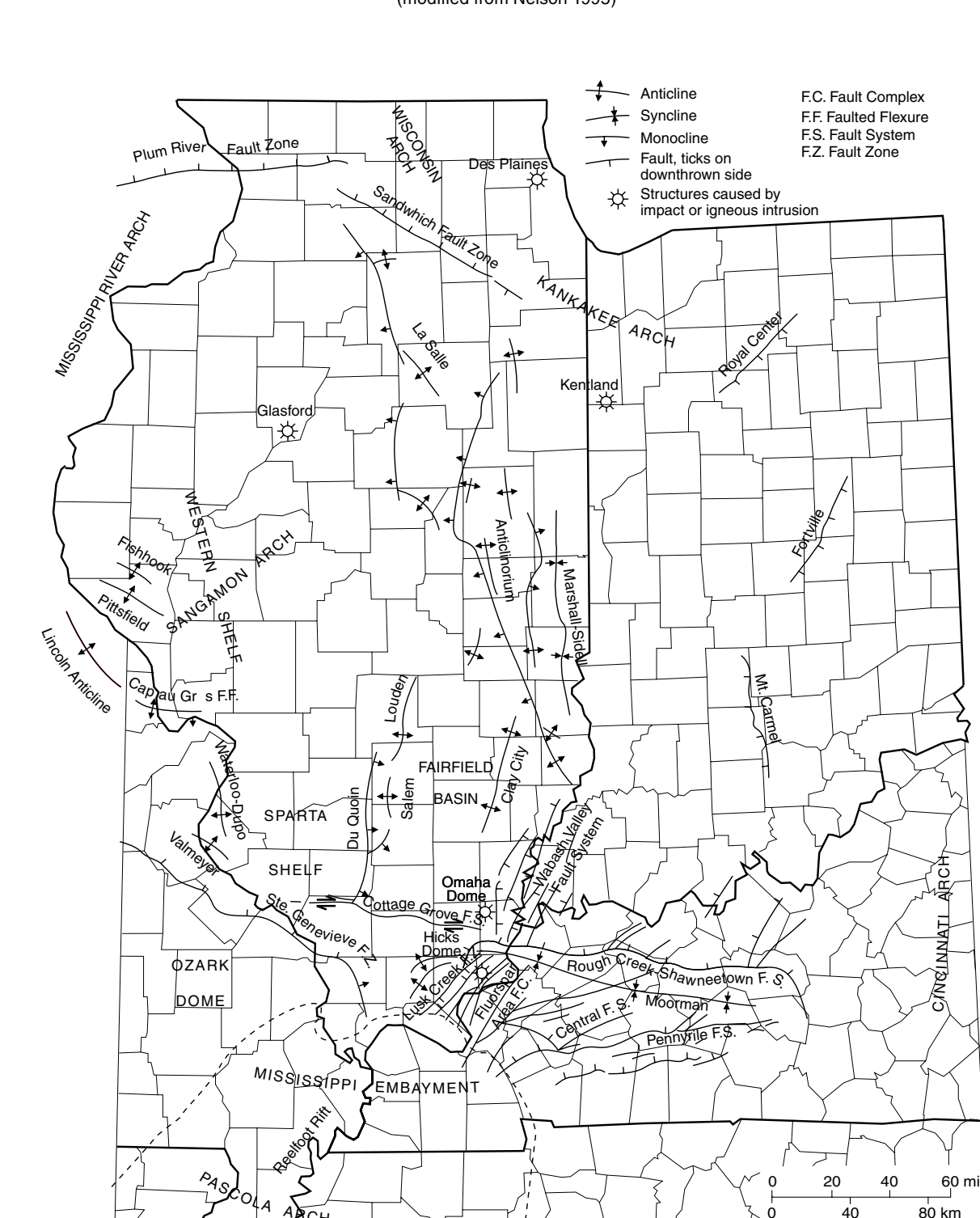
Structural Features of Illinois
