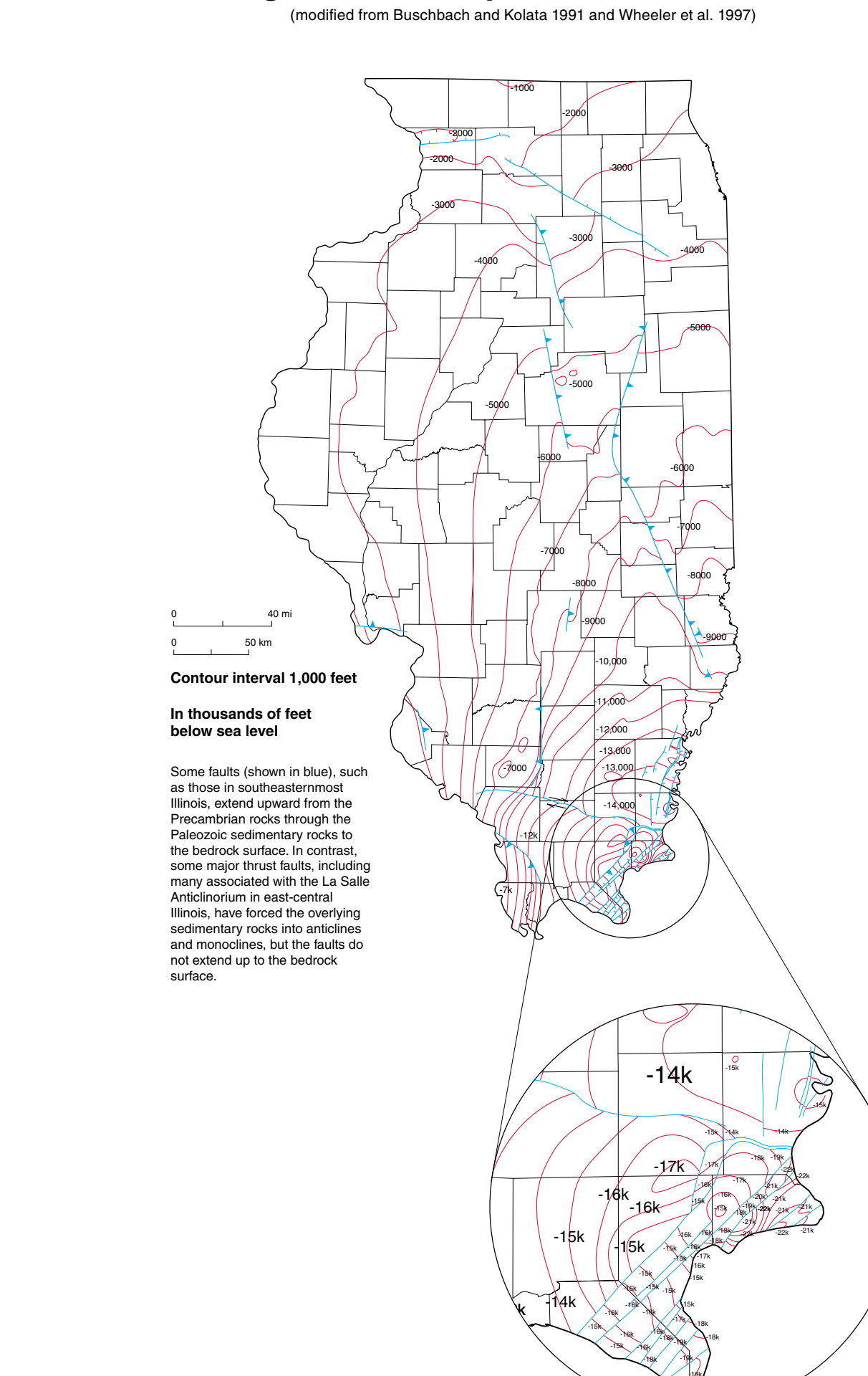
Configuration of Top of Precambrian Rocks
