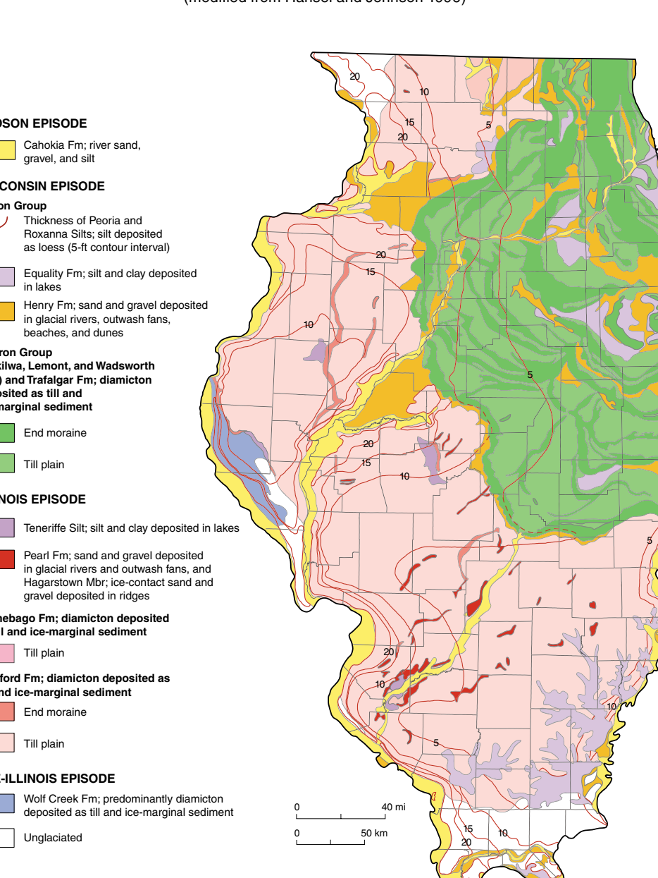
Quaternary Geology of Illinois
