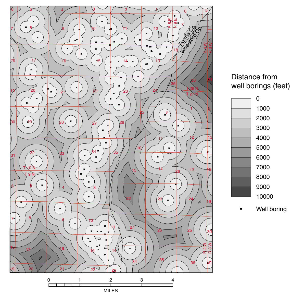
Figure 2 Well data distribution map. Data points are surrounded by 1,000-foot contours, indicating the relative reliability of the bedrock surface elevations interpreted between the data points.
