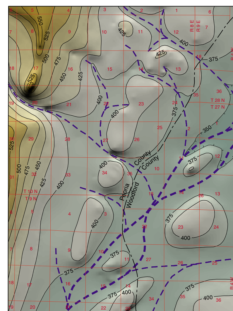
Figure 1 Shaded relief map of the bedrock surface. Superimposed contours have an interval of 25 feet. Note that the western side of the bedrock valley is about 1 to 2 miles west of the modern western valley wall. Blue dashed lines indicate the fluvial drainage patterns prior to the onset of Quaternary glaciation. The thicker lines mark the southwest-trending main channel of the ancient river valley; thinner lines indicate tributaries. Although the lowest elevations of the bedrock surface (hachured contour) within the quadrangle are in the upstream part of the main channel, regional analysis indicates that flow was to the southwest.
