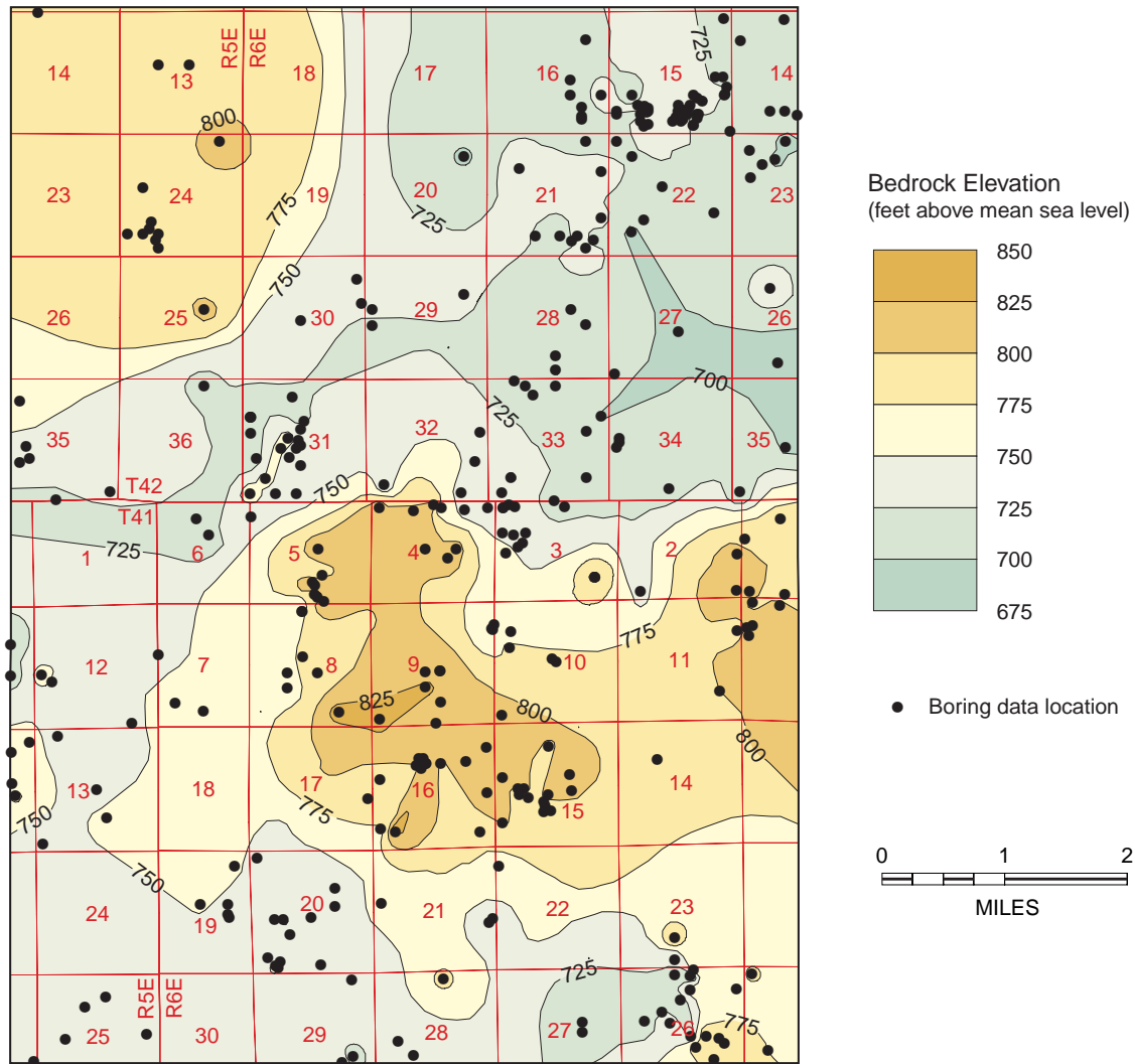
Figure 5 Bedrock topography of the Hampshire Quadrangle.
