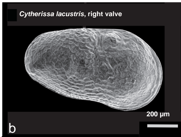
Figure 11 Examples of fossils recovered from boring 35696 (Sec. 9, T41 N, R6E) (a) leaf of Salix herbacea (snowbed willow) and (b) Cytherissa lacustris , an ostracode.
