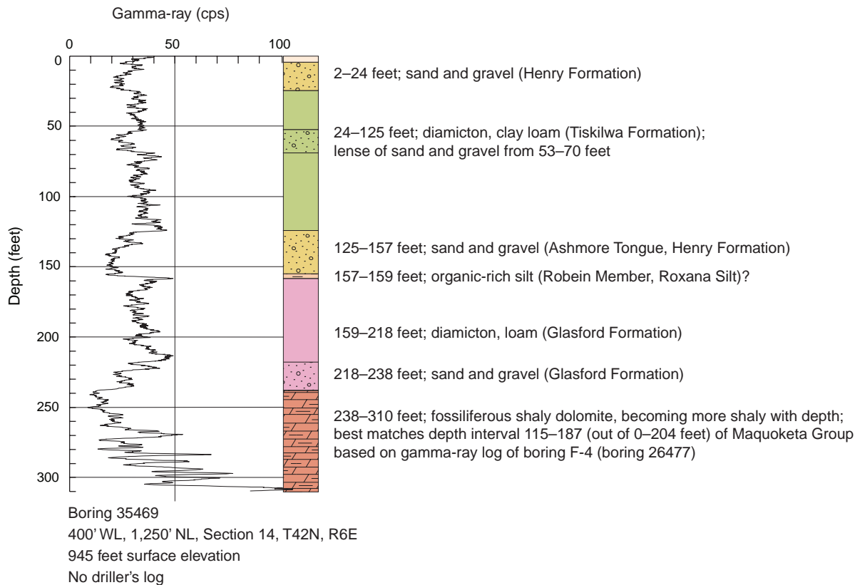
Figure 8 Lithologic and gamma-ray log of boring 35469 (NW Sec. 14, T42N, R6E) located 1.5 miles north and 1 mile east of Hampshire. This boring is used in cross section A-A' on map sheet 2. cps, counts per second.
