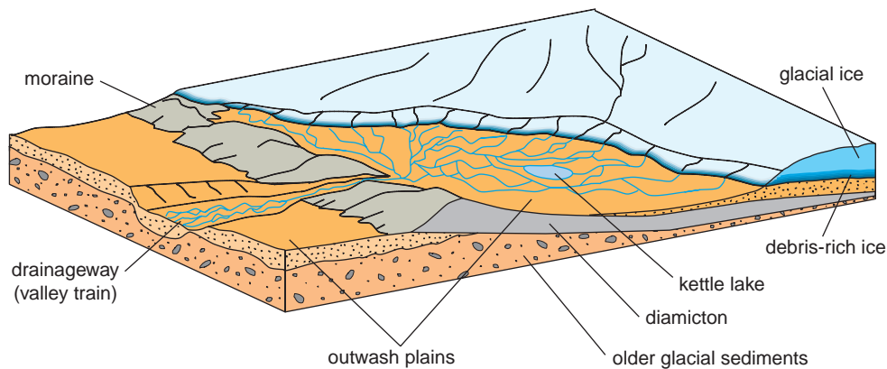
Figure 2 Conceptual model of landform-sediment assemblages associated with the margins of continental glaciers (from Curry et al. 1997).
