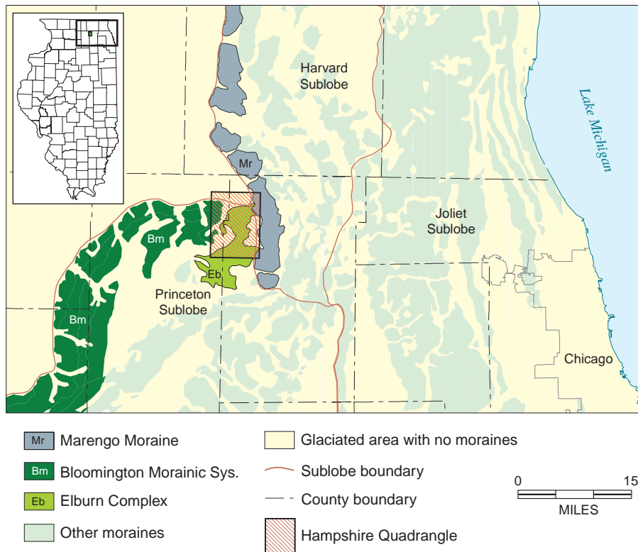
Figure 1 Wisconsin Episode moraines in northeastern Illinois. Moraines, shown in gray and green, were formed near the terminus of glacial ice at various positions of the Lake Michigan Lobe. Glaciers advanced in a westerly and southwesterly direction into Illinois from the Lake Michigan basin. The oldest moraines occur generally to the west and the younger moraines to the east. In the area of the last glaciation, the yellow areas are typically drainageways or plains of outwash, lake sediment, or till. This map is adapted from Willman and Frye (1970) and Hansel and Johnson (1996). The Hampshire Quadrangle is hachured in red.
