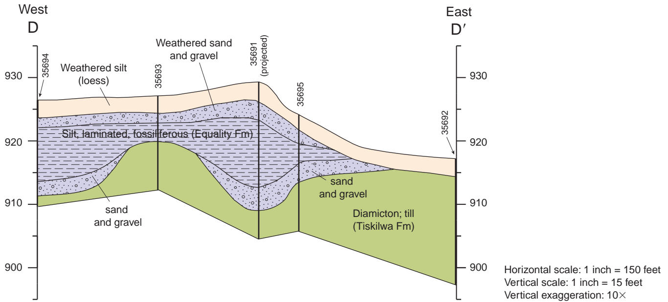
Figure 10 Cross section across part of an ice-walled lake deposit 1 mile west of Burlington. The line of section is shown on figure 9a.
