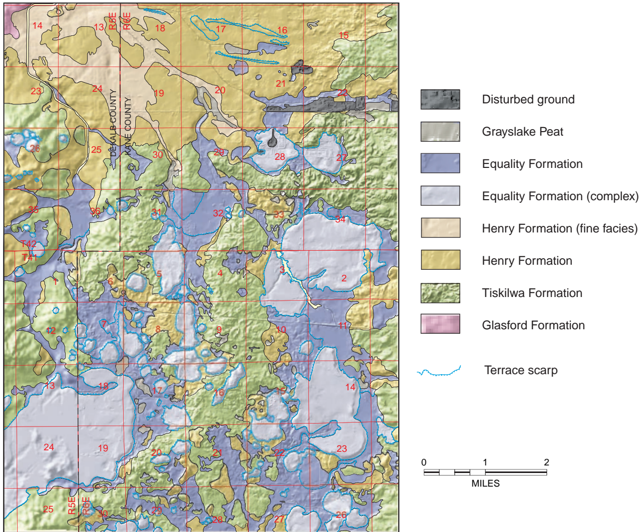
Figure 6 The surficial geology draped over the shaded relief map of the 10-foot DEM of Kane County and 30-meter DEM of DeKalb County. The high terraces (light purple), formed of laminated lake sediment sandwiched by thin layers of sand and gravel, stand out against the lower terraces (dark purple), formed of fine-grained lake sediment. The high terraces were formed in ice-walled lakes and the low terraces in slackwater lakes.
