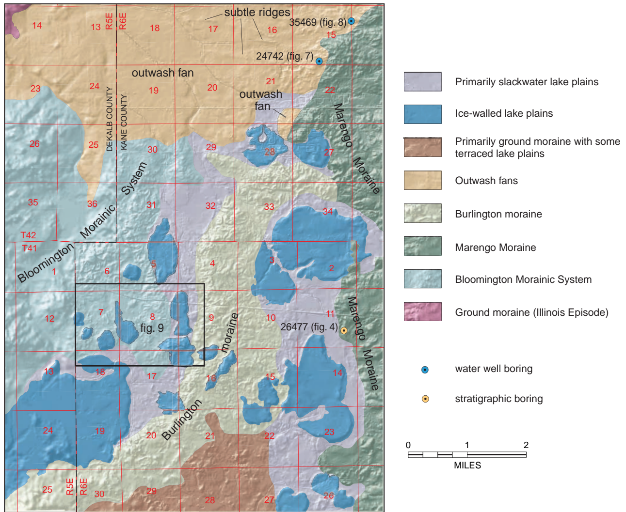
Figure 3 Shaded relief map of the Hampshire Quadrangle, from a 10-foot resolution DEM (derived from 2-foot contours) of Kane County and a 30-meter DEM of DeKalb County. Formal names include the Marengo Moraine and Bloomington Morainic System. The Burlington moraine is informal. The locations of borings shown in figures 4, 7, and 8 are shown. The box shows the location of figure 9.
