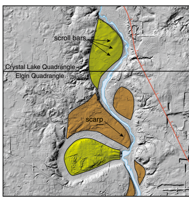
Figure 3 Location of large point bars and erosional terraces along the Fox River in Kane County in the southern part of the Crystal Lake Quadrangle and northern part of the Elgin Quadrangle. The scroll bars evident on the large point bar may be related to the scarps on the erosional terrace immediately to the south. The Fox River has eroded at least 50 feet into the highest parts of these landforms. The maximum extent of the Harvard Sublobe during the Woodstock Phase is shown in brown. Modified from Curry et al. (1999).
