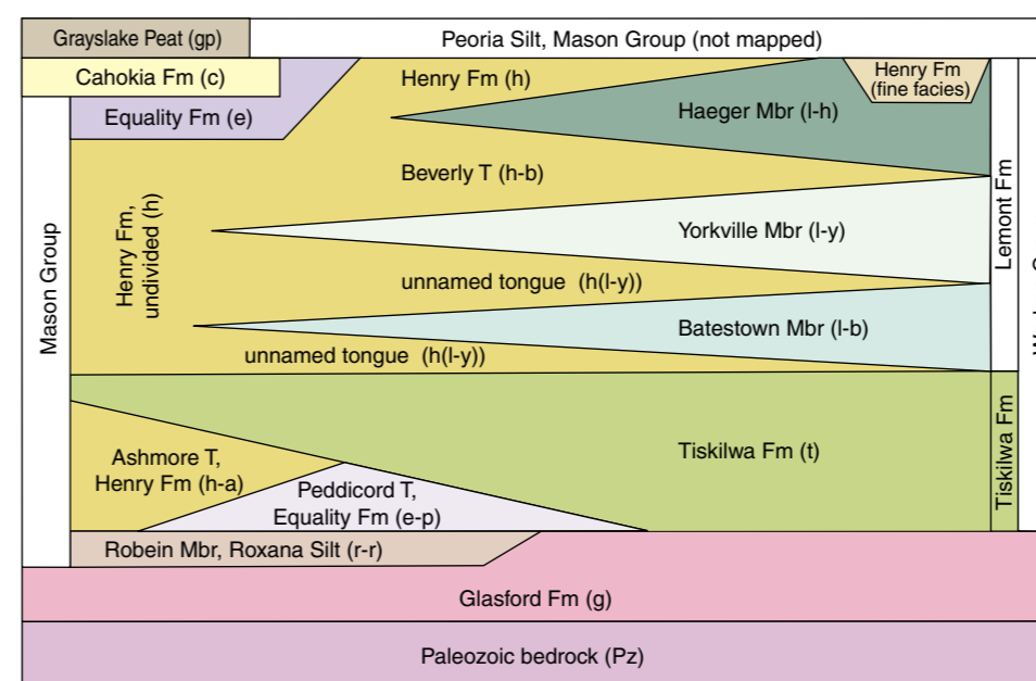
Figure 5 Schematic representation of the spatial relationships among the lithostratigraphic units and associated tongues.
