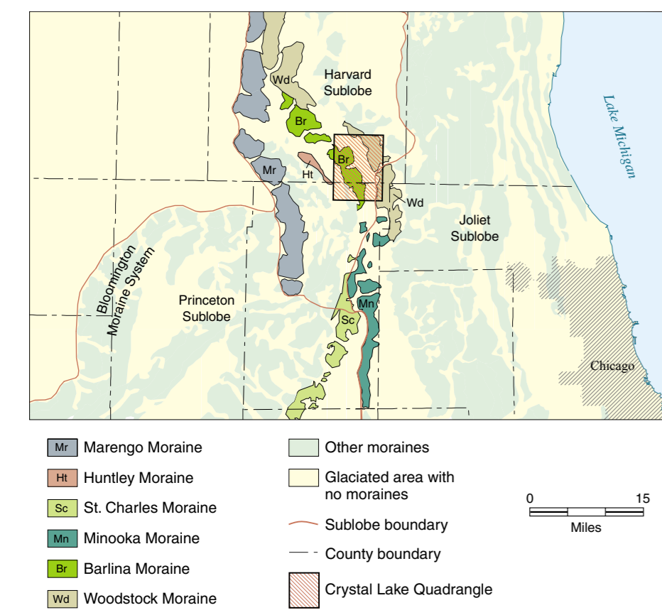
Figure 1 Wisconsin Episode moraines in northeastern Illinois. Moraines were formed near the terminus of glacial ice at various positions of the Lake Michigan Lobe. Glacial ice advanced in a westerly and southwesterly direction into Illinois from the Lake Michigan basin. The older moraines of this figure generally occur to the west and the younger moraines to the east. In the area of the last glaciation, the yellow areas are typically drainageways or plains of outwash, lake sediment, or till. Adapted from Willman and Frye (1970) and Hansel and Johnson (1996).
