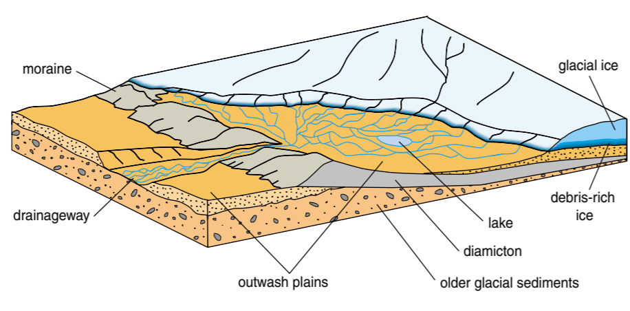
Figure 2 Conceptual model of landform and sediment assemblages associated with the margins of continental glaciers (Curry et al. 1997).
