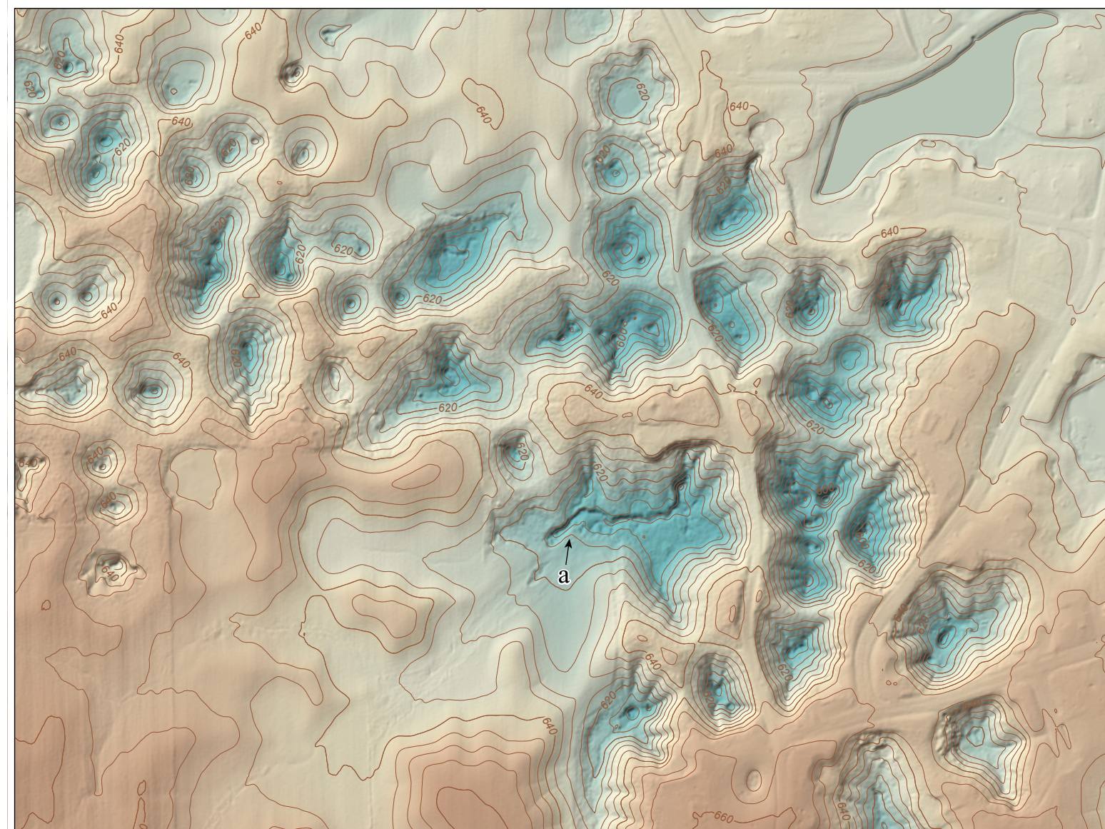
Figure 2 LiDAR digital terrain model (DTM) showing an area of approximately 0.25 square mile exhibiting a high density of sinkhole features, ranging in depth from about 20 feet to more than 50 feet (T35S, R10W). A DTM represents only the ground surface and is extracted from airborne LiDAR data using automated filtering methods to produce what is commonly referred to as a "bare-earth" point cloud. Monroe County is located in southwestern Illinois within the Sinkhole Plain, which contains the highest concentration of karst features within the state. It is estimated that the region contains more than 10,000 sinkhole features, making them distinctive landscape elements within the county. Sinkholes begin with the collapse of unconsolidated sediments into a bedrock crevice or cavity, and because the entire region is underlain by highly erodible limestone, geologic conditions are optimal for sinkhole creation. Disappearing streams are another characteristic feature of karst terrain, and an example is shown at (a). Contour interval is 5 feet. Scale is 1:4,800 (1 in. = 400 ft).
