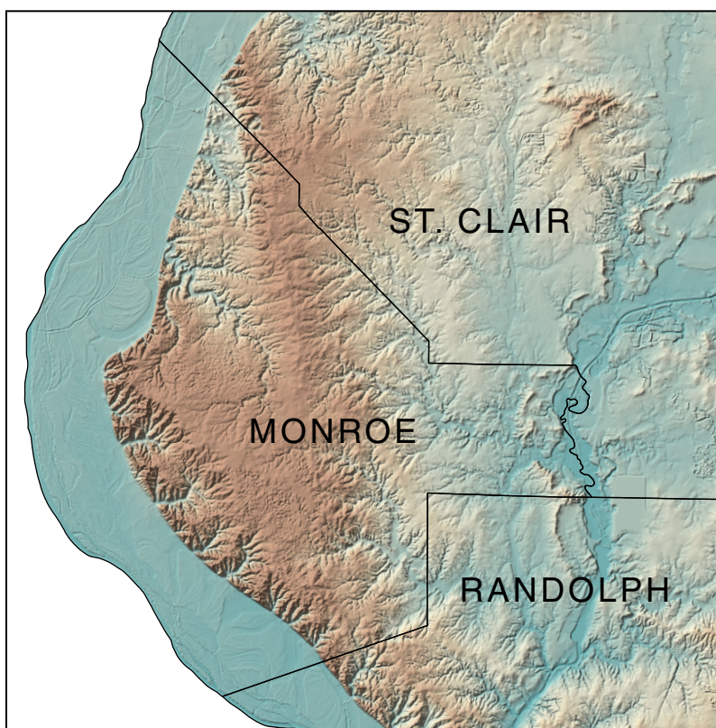
Figure 4 Generalized surface topography for a portion of southwestern Illinois produced from the U.S. Geological Survey, one-third arc second resolution National Elevation Dataset (U.S. Geological Survey 2014).
